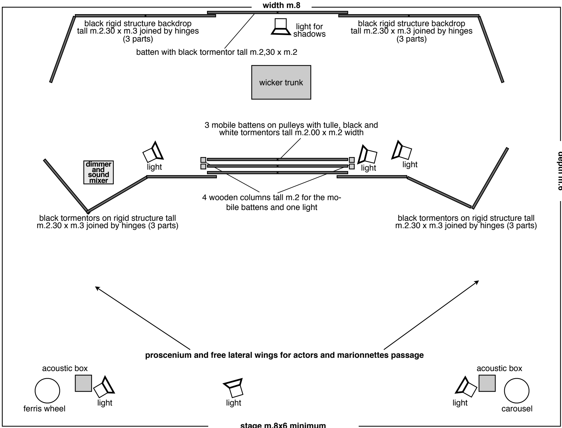
PETROUCHKA stage and light plan
