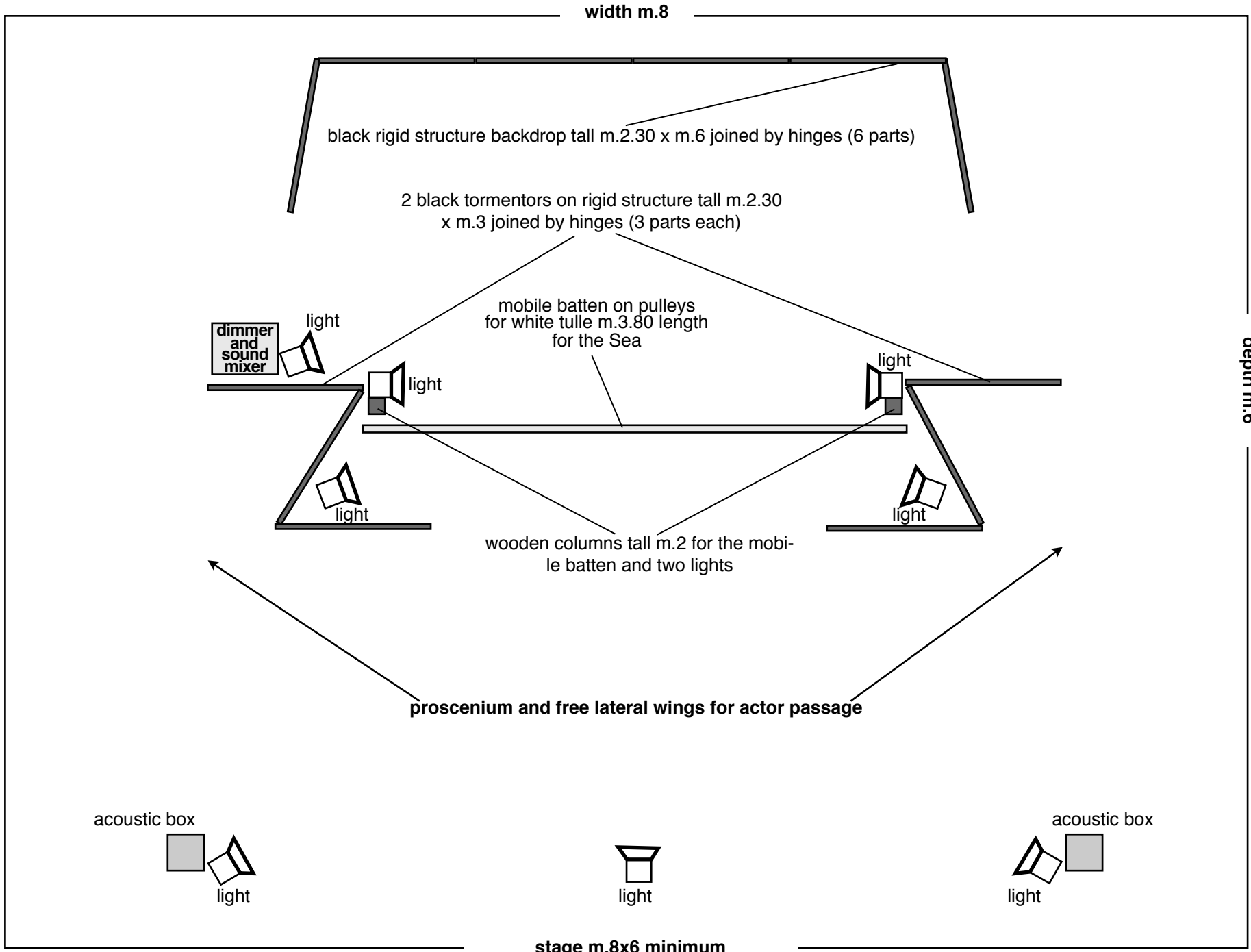
AZZURRA BALENA stage and light plan
